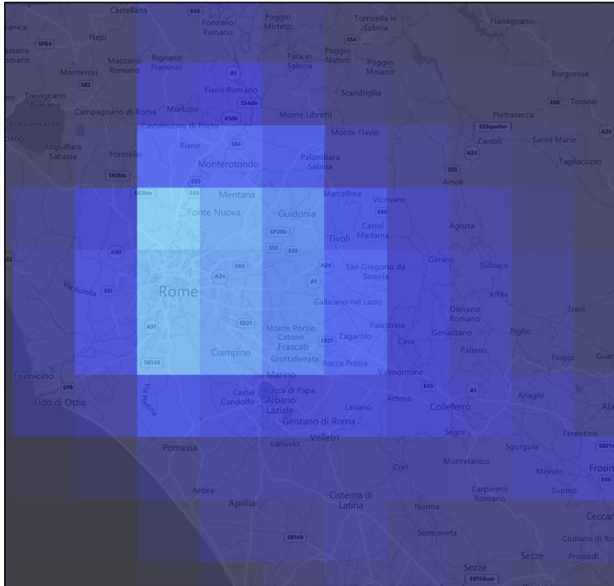
CAMS Regional, NO 2 , Rome
