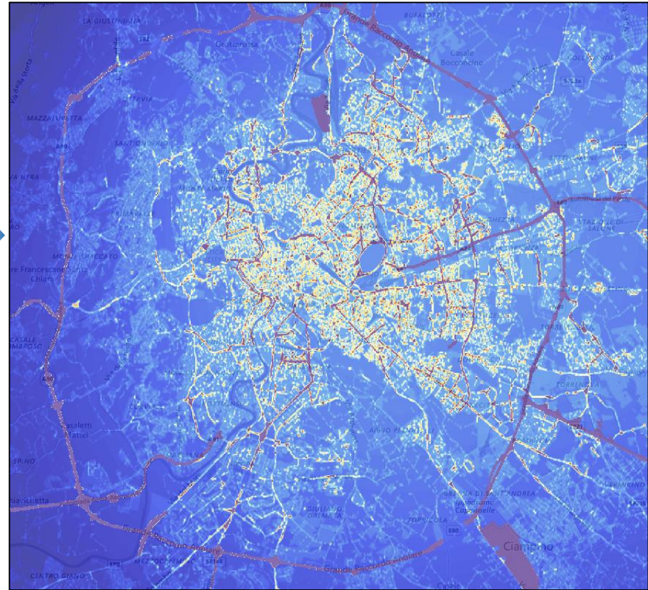
AIR-Portal, 100m, NO 2 , Rome
